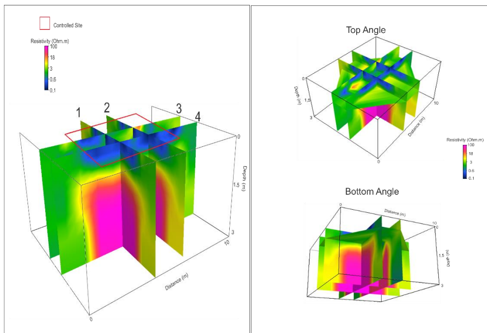
Figure 6: Sections in 3D of Resistivity.
