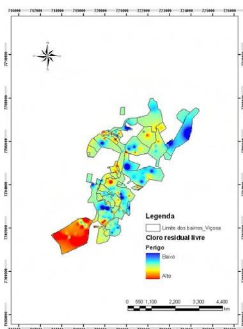
a) Cloro residual livre - mg/L.
